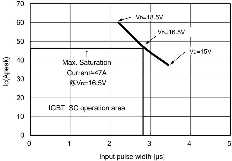
Fig.3-1-15 Typical SCSOA curve of SLIMDIP-S
