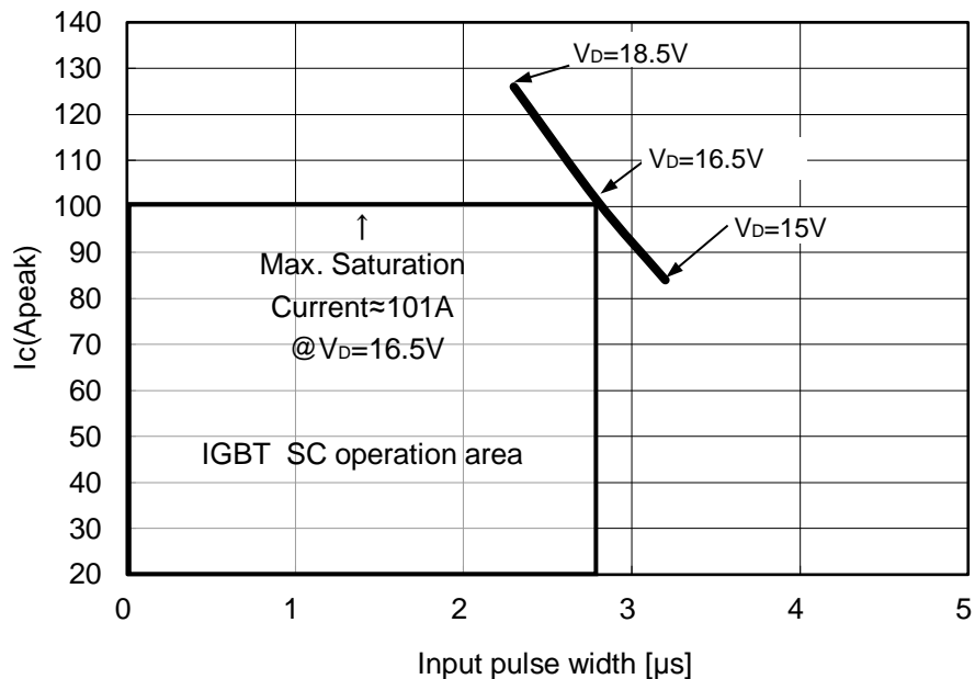
Fig.3-1-16 Typical SCSOA curve of SLIMDIP-L
