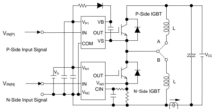
Fig.2-1-6 Evaluation circuit (inductive load)
