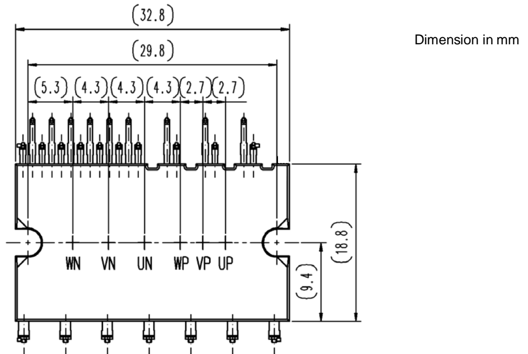
Fig.2-1-3 Power chip position
