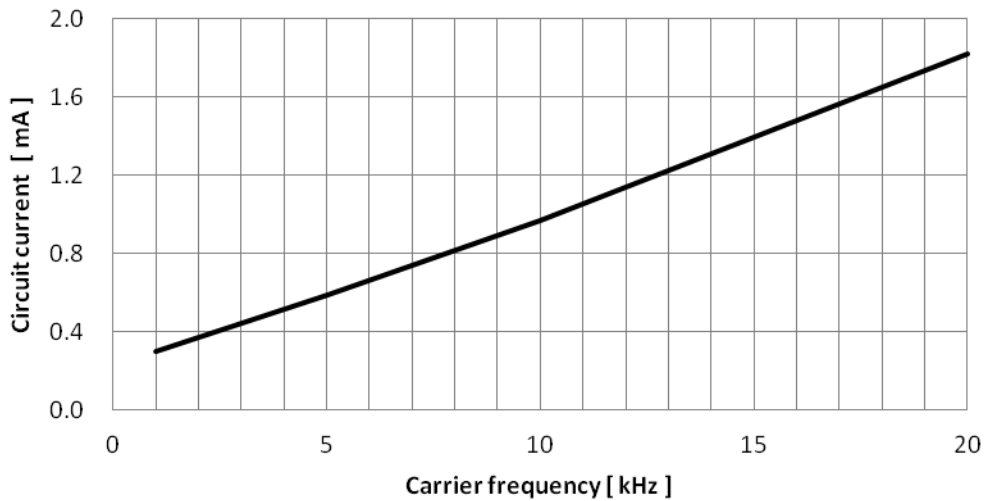
Fig.4-2-2 I_{DB} vs. Carrier frequency for SLIMDIP-L
