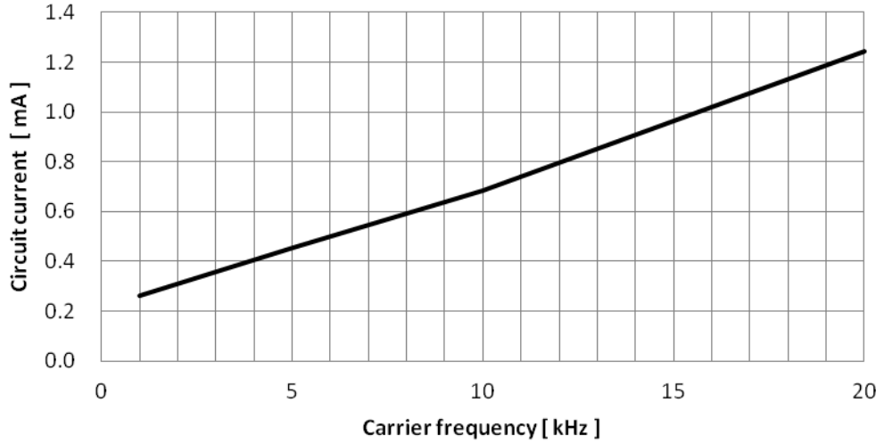
Fig.4-2-1 I_{DB} vs. Carrier frequency for SLIMDIP-S
