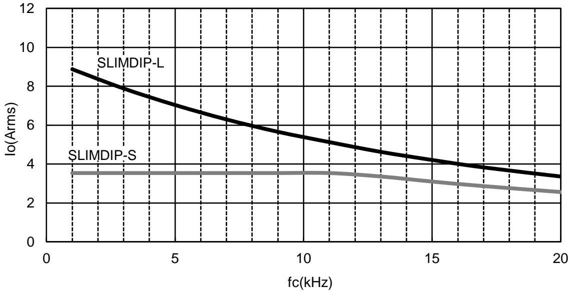
Fig.3-2-2 Effective current-carrier frequency characteristic s(Typical)
