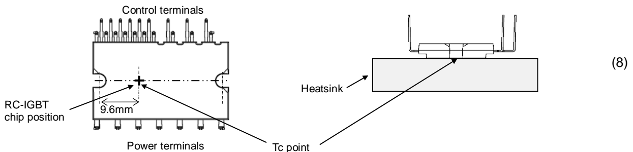
Fig.2-1-1 T_C measurement position
