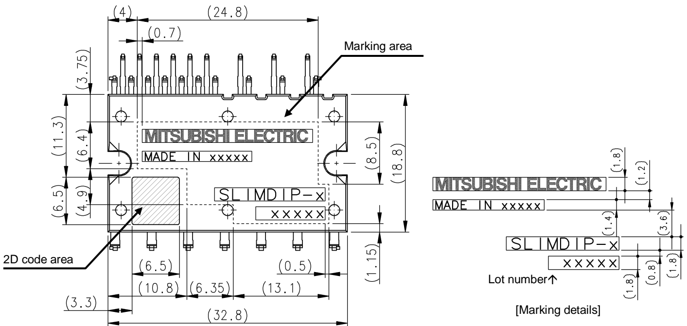
Fig.2-3-2 Laser marking view
